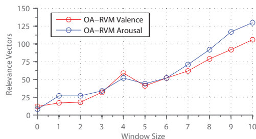
Fig. 4. Increase of Relevance Vectors in the OA model with the increase of window size in output features (Subject 1, Positive). The RVM RV are 643 and 626 for valence and arousal respectively.
