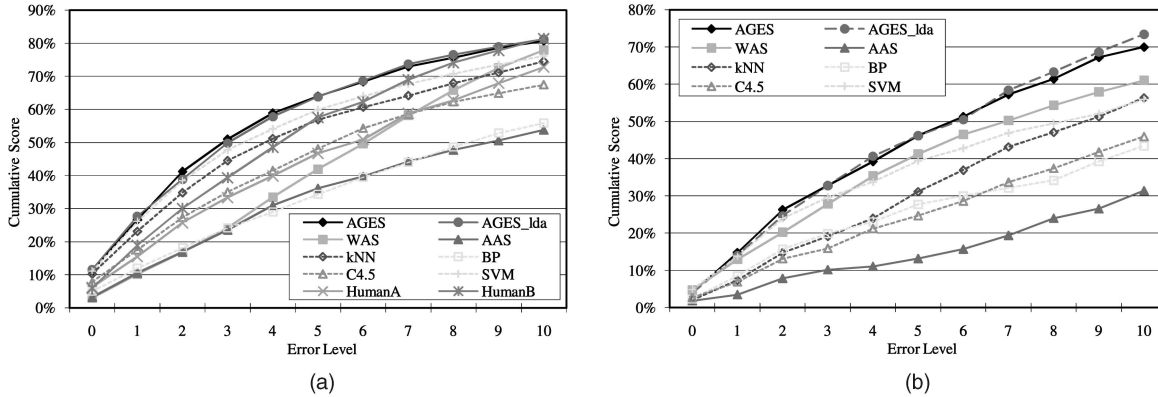
Fig. 4. Cumulative scores of standard age estimation on (a) FG-NET (LOPO) and (b) MORPH (Test Set).
