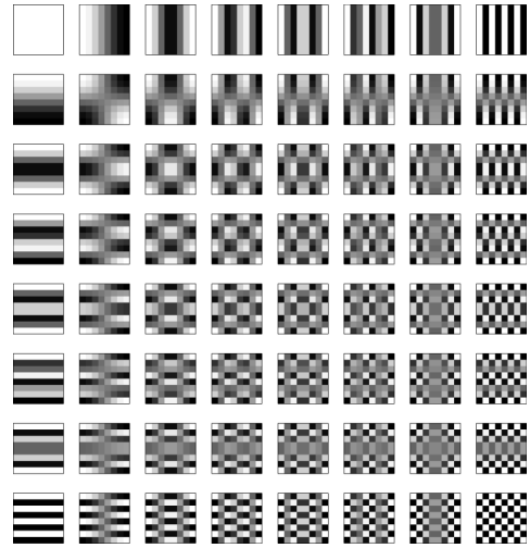
Figure 1. DCT basis functions for N = 8 . (0, 0) is at the top left corner.
